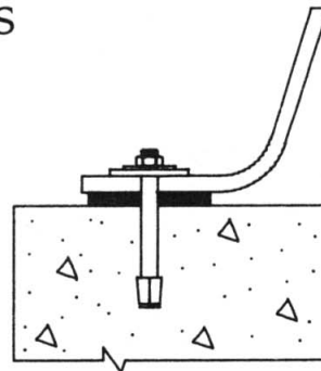
TYPICAL BASE DETAIL
